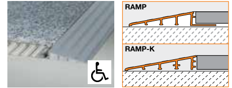
1.8 Schluter®-RENO-RAMP/-K
