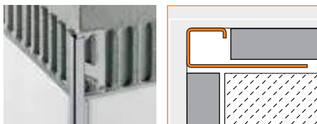
2.10 Schluter®-QUADEC
