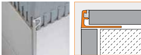
2.3 Schluter®-JOLLY
